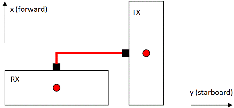
Figure 1 Typical EM 2040 transducer configuration viewed from above (single RX)
